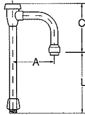
GROUP NO. 3 Angle VB Gooseneck
